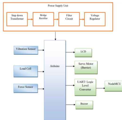
Fig .3 Block Diagram
