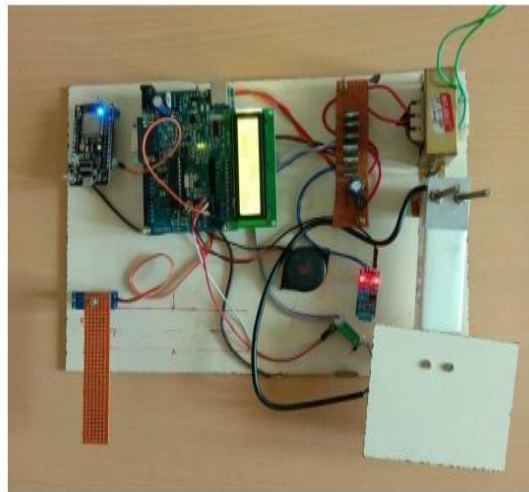
Fig. 4 Prototype Model
